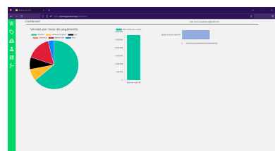
Dashboard
