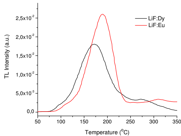
Figure 4. Typical TL emissions of LiF:Dy and LiF:Eu composites sintered at 750°C beta irradiated (11 Gy, ^{90}\text{Sr}+^{90}\text{Y} ).
