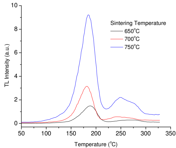
Figure 2. Typical TL emissions of LiF:Nd composites sintered at 650, 700 and 750°C beta irradiated (22.6 Gy, ^{90}\text{Sr}+^{90}\text{Y} ).
