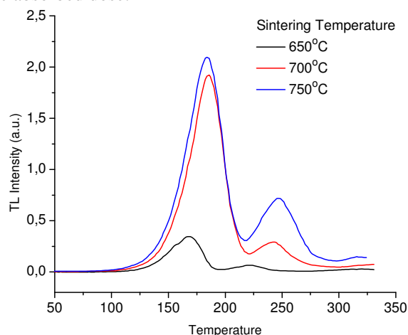
Figure 1. Typical TL emissions of LiF composites sintered at 650, 700 and 750°C beta irradiated (22.6 Gy, ^{90}\text{Sr}+^{90}\text{Y} ).
