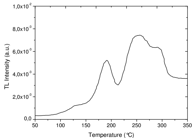
Figure 5. Typical TL emissions of LiF:Tb composite sintered at 750°C beta irradiated (11 Gy, ^{90}\text{Sr}+^{90}\text{Y} ).
