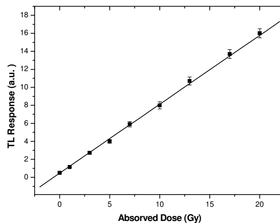
Figure 3. TL response of LiF:Nd composites sintered at 750°C beta irradiated in the range from 0.1 to 16 Gy.
