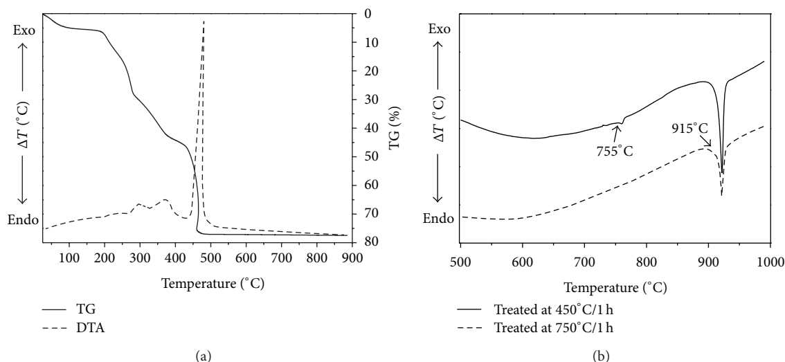
FIGURE 1: (a) Simultaneous DTA/TG curves of the resin dried at 100^{\circ}\text{C}/24\text{ h} . (b) DTA curves obtained after thermal treatments at 450^{\circ}\text{C}/1\text{ h} and 750^{\circ}\text{C}/1\text{ h} .
