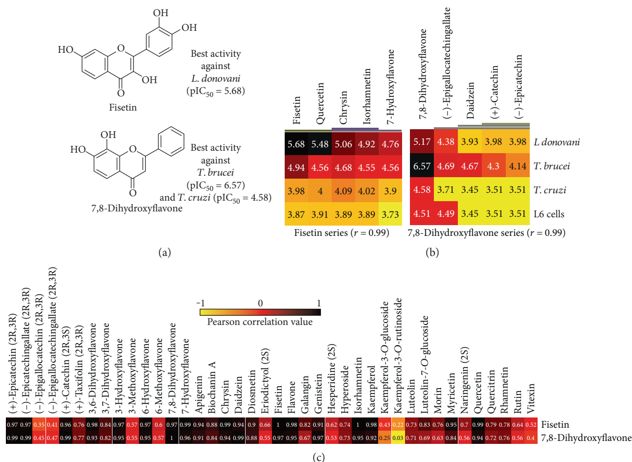
FIGURE 4: Results of hierarchical clustering analyses carried out in Gitoools 2.3.1 using Euclidean distance and correlation analysis with the most active flavonoids. (a) The most active compounds: fisetin against L. donovani and 7,8-dihydroxyflavone against T. brucei and T. cruzi . (b) The most relevant part of HCA cluster based on \text{pIC}_{50} of all flavonoids. (c) Correlation values of the 40 flavonoids studied with the more active compounds. The intensity of the colors in the heatmap is according to the \text{pIC}_{50} values.
